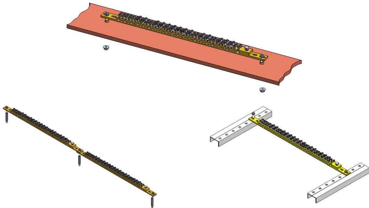
Fixing on copper bars, on profiles and on extensions
